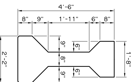
END VIEW (Type IV P.C.B.)
