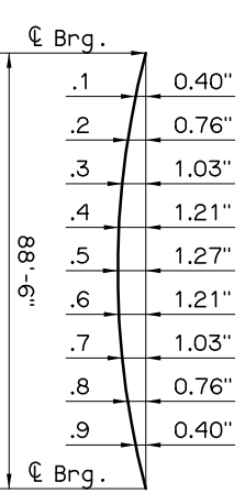
DEAD LOAD DEFLECTION DIAGRAM
