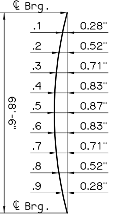
DEAD LOAD DEFLECTION DIAGRAM
