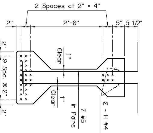
END SECTION
