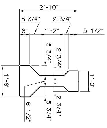
END VIEW (Type B P.C.B.)
