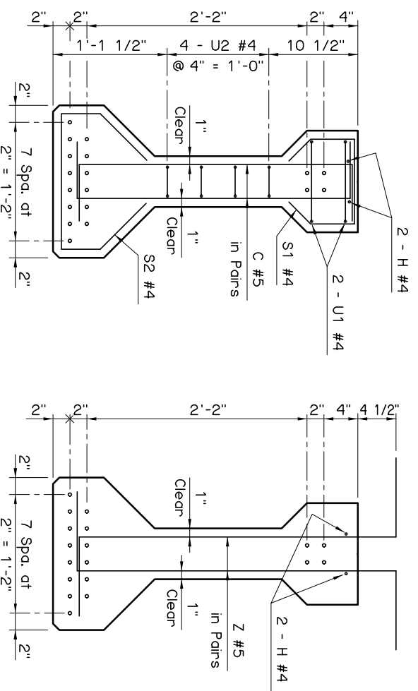
BEAM SECTIONS (18 - 0.6"Ø STRANDS)
