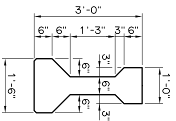
END VIEW (Type II P.C.B.)
