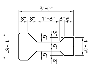
END VIEW (Type II P.C.B.)
