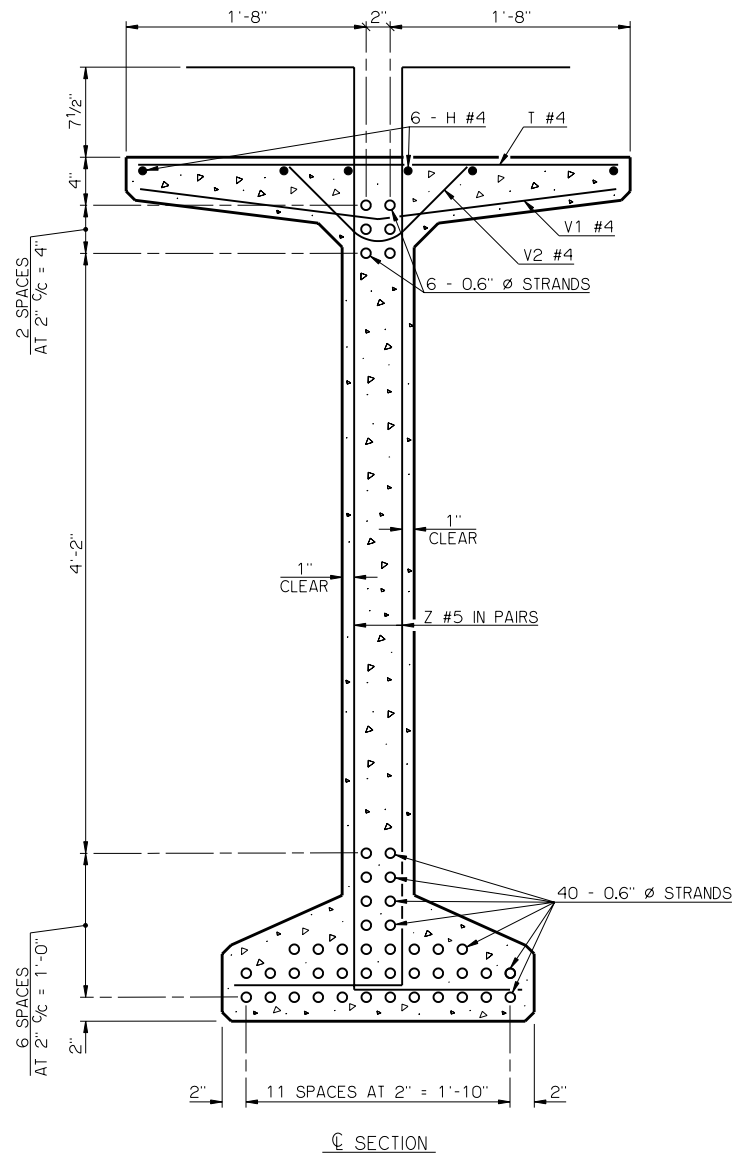
BEAM SECTIONS (46 - 0.6" Ø STRANDS)
