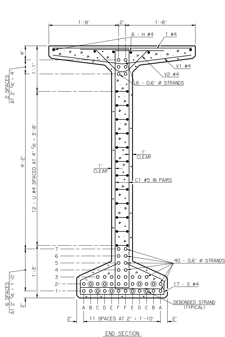
BEAM SECTIONS (46 - 0.6" Ø STRANDS)
