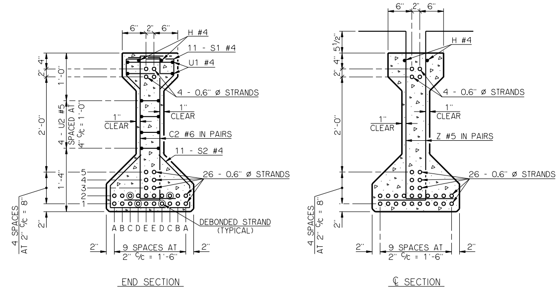
BEAM SECTIONS (30 - 0.6" STRANDS)
