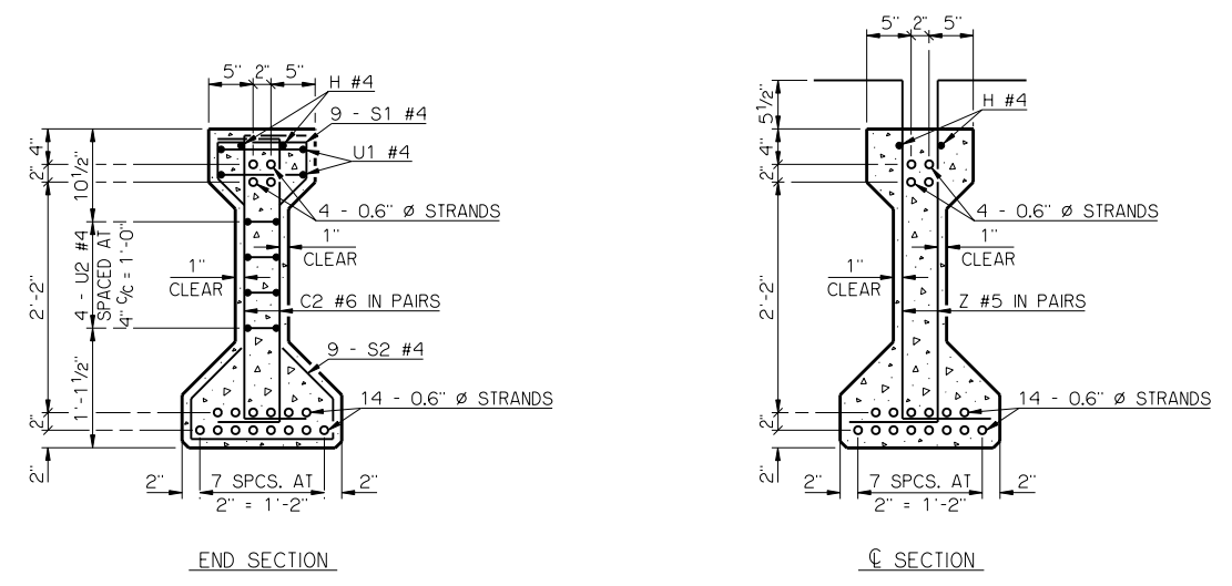
BEAM SECTIONS (18 - 0.6" \phi STRANDS)
