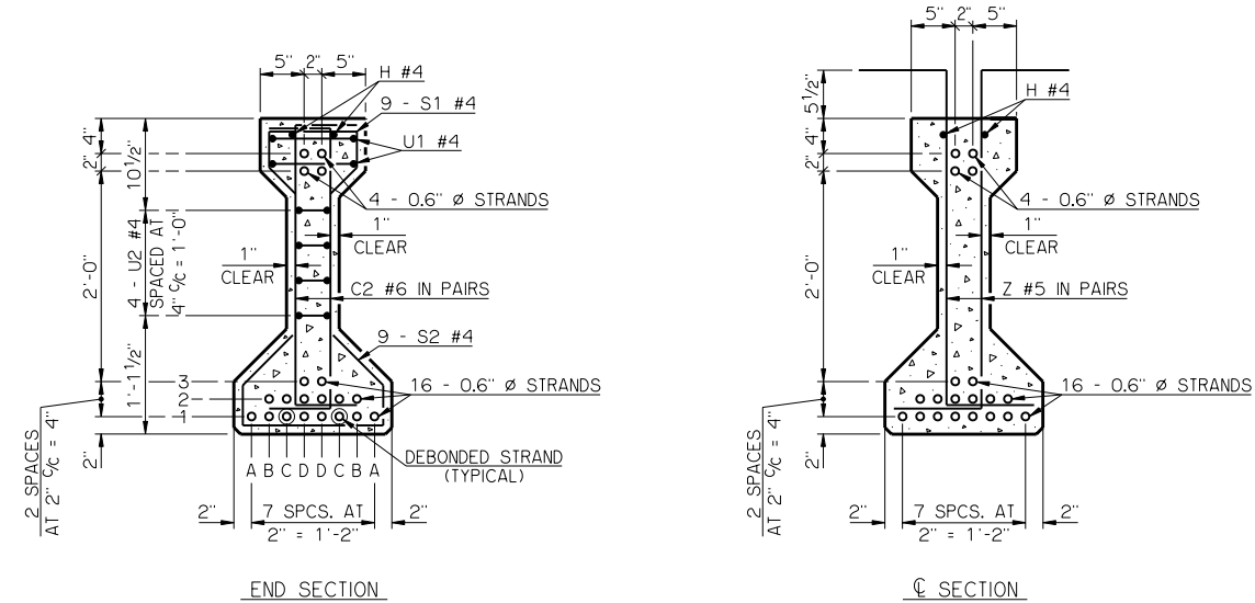
BEAM SECTIONS (20 - 0.6" \varnothing STRANDS)
