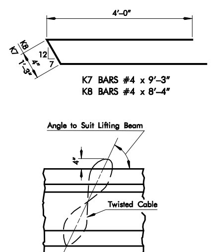
DETAIL OF LIFTING EYE
