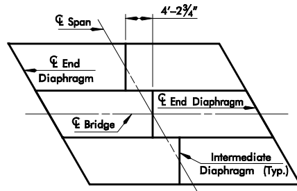
TYPICAL DIAPHRAGM SPACING - 30° SKEW
