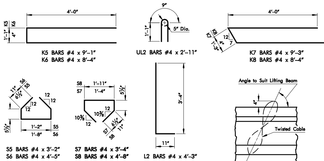
DETAIL OF LIFTING EYE
