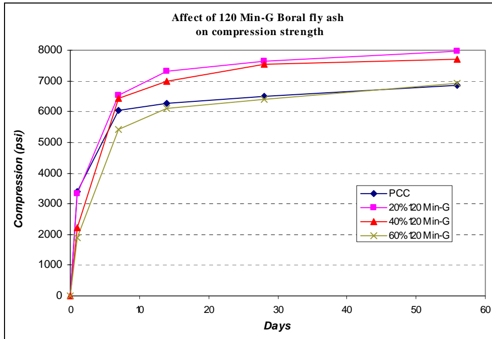
Figure 5.43 Effect of fly ash content on 120 minutes ground Borol fly ash concrete
