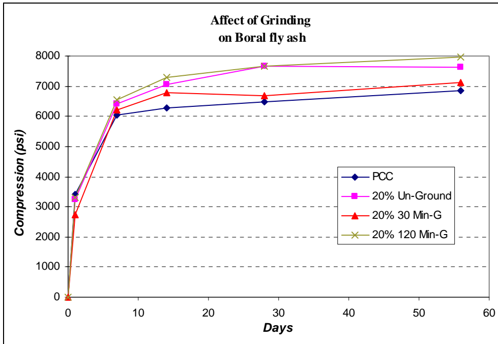
Figure 5.23 Effect of grinding duration on 20% Boral fly ash concrete
