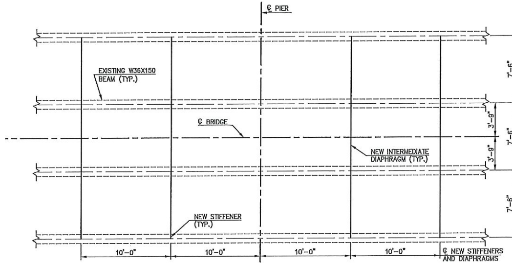
PARTIAL PLAN AT PIER NO. 1 & PIER NO. 2
