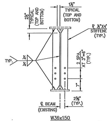
INTERMEDIATE DIAPHRAGM STIFFENER DETAIL
