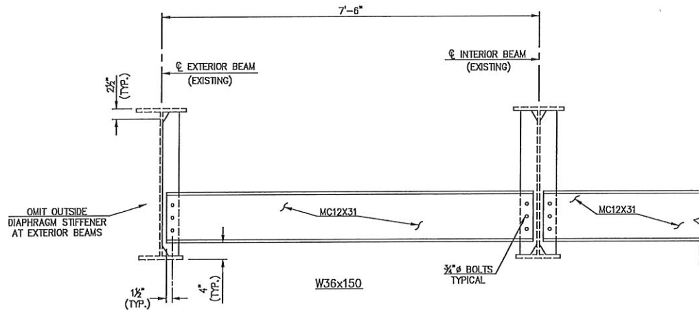
INTERMEDIATE DIAPHRAGM ELEVATION
