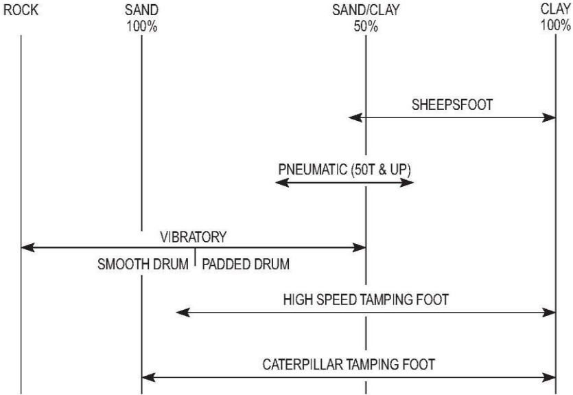
RANGES OF SOIL TYPES FOR SOIL COMPACTION EQUIPMENT
